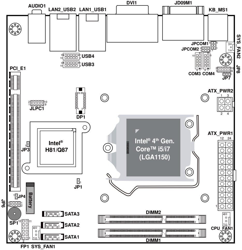
BM-0942 Front Connector, Jumper and Component locations
