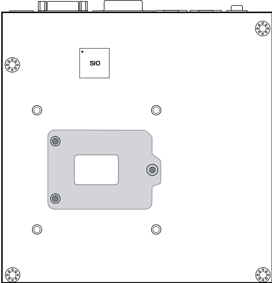
BM-0942 Rear Component locations
