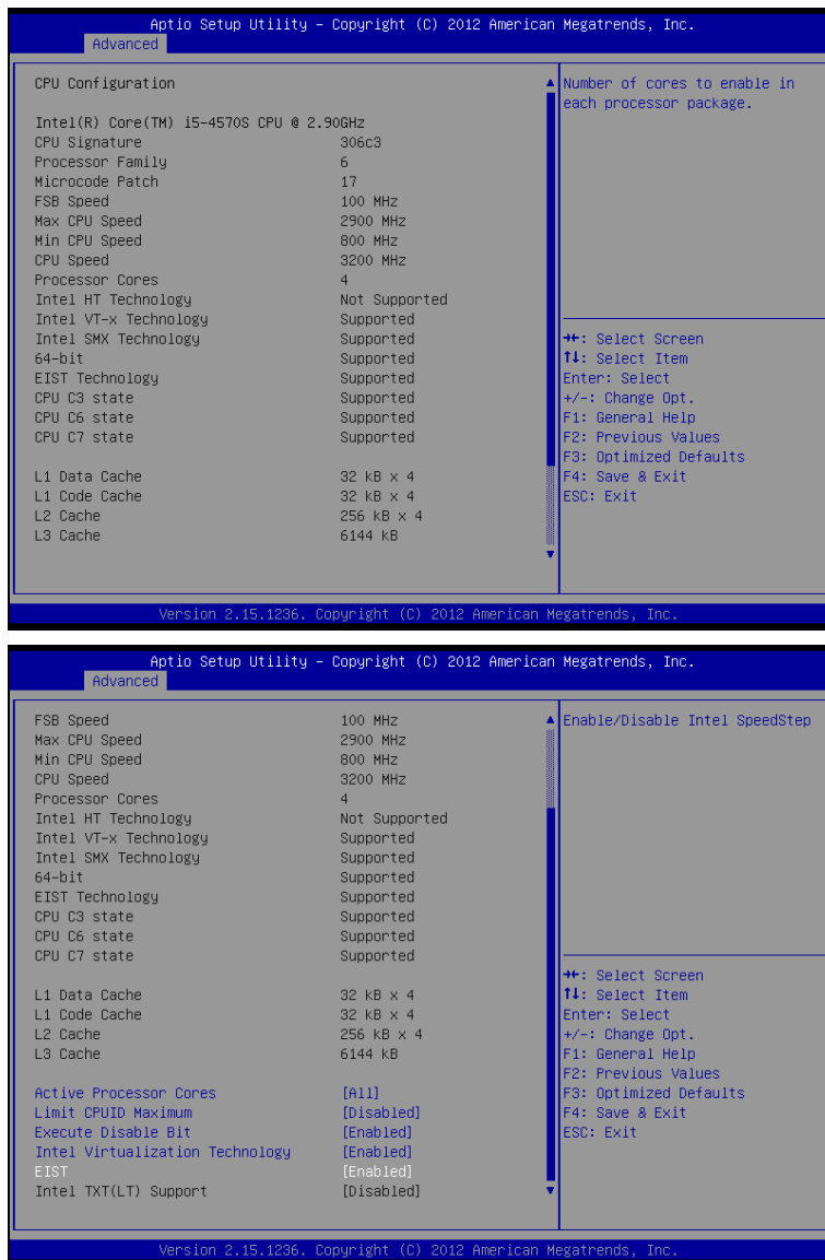
CPU configuration screen
