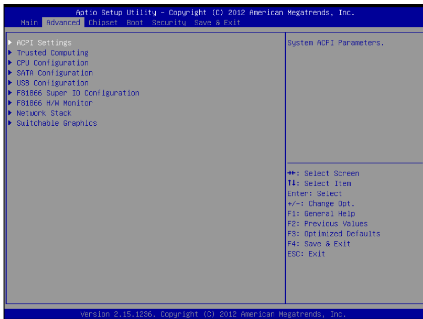
Advanced screen
