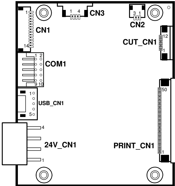
MB-1030TD, TE Printer Board Component Locations
