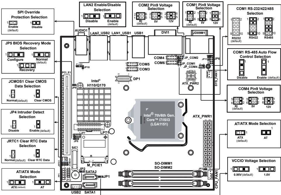
Figure 3-1. Main Board Component Location (Top View)
