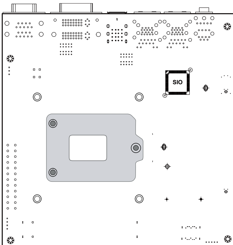
Figure 3-2. Main Board Component Location (Bottom View)
