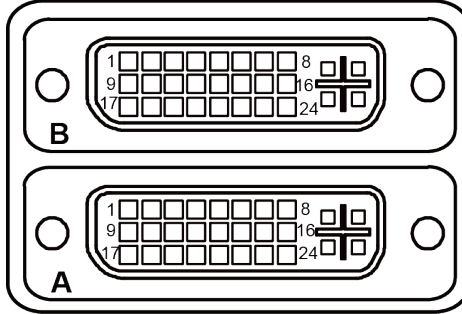
DVI1 connector signals (A):
