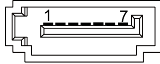
SATA1
