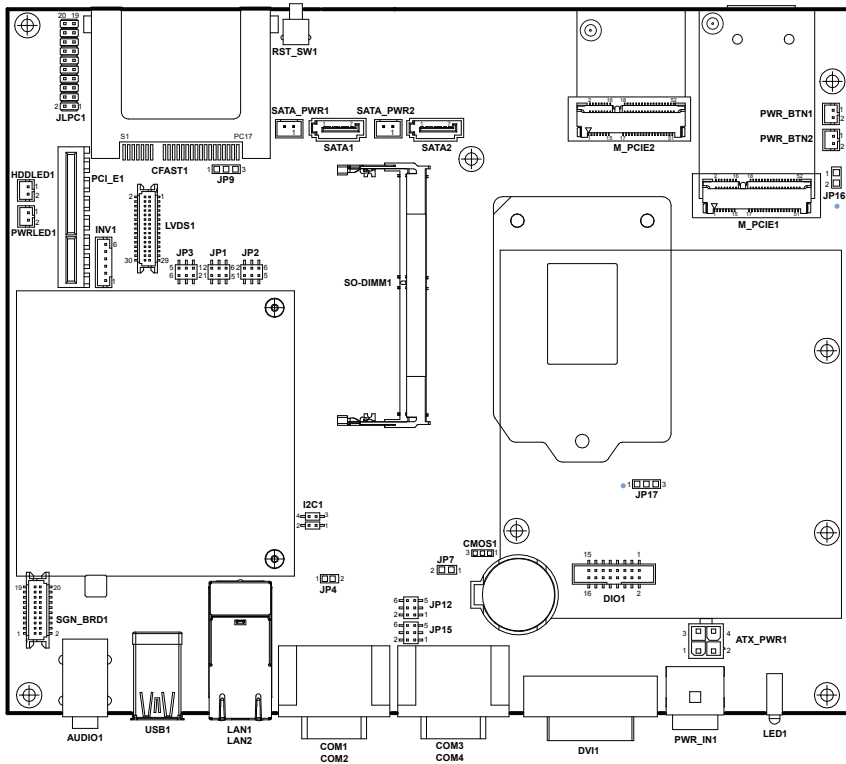
Figure 3-1. Main Board Component Location (Top View)
