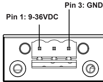
DC IN
