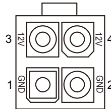
ATX_PWR1
