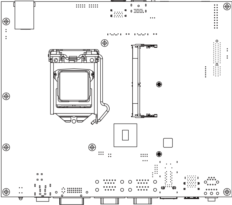
Figure 3-2. Main Board Component Location (Rear View)
