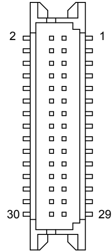
LVDS1
